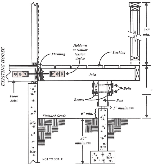
TYPICAL DECK SIDE VIEW DIAGRAM
