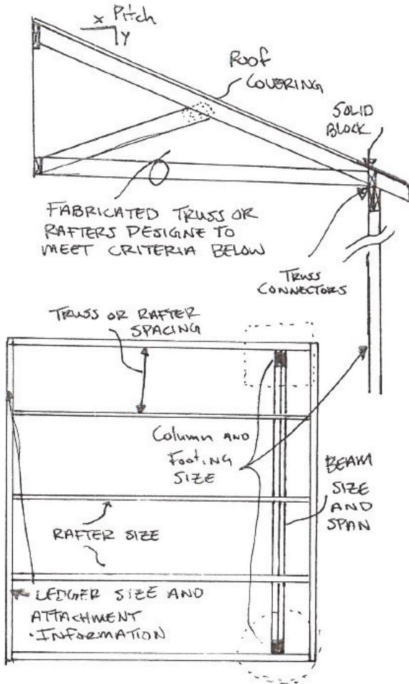
DETAIL 'A'
